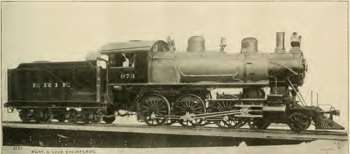
BALDWIN PASSENGER 4-6-0 FOR THE ERIE.
